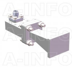
LB-42-10-C-SFSPO Standard Gain Horn Antenna 18-26.5GHz 10dB Gain SMA Female
